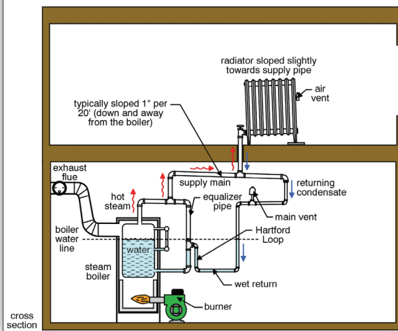
One pipe parallel flow system
