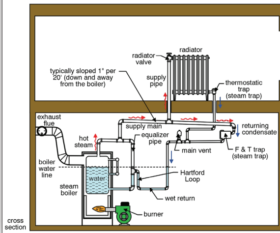
Two pipe system
