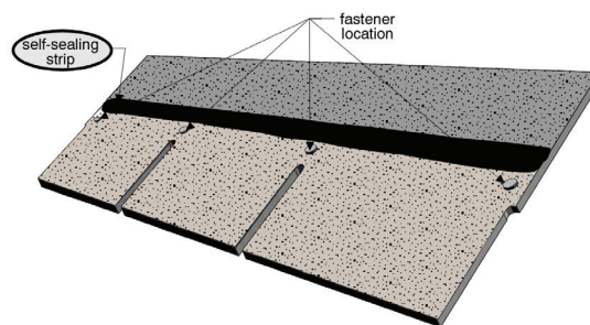
Self-sealing tabs
