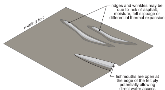
Ridging and fishmouths on flat roofs
