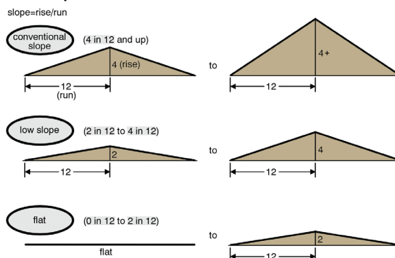
Roof slopes
