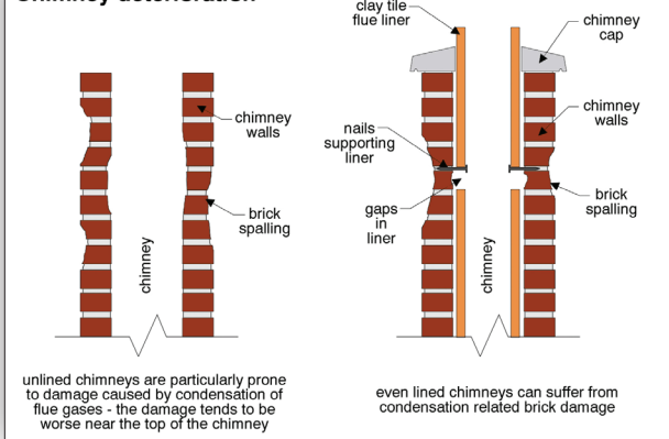
Chimney deterioration
