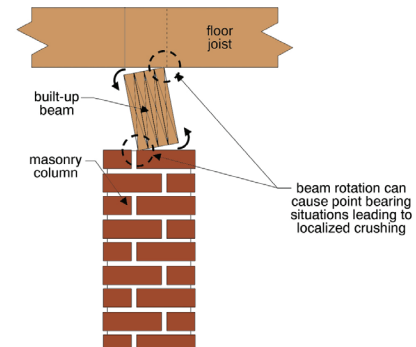
Rotated or twisted beams
