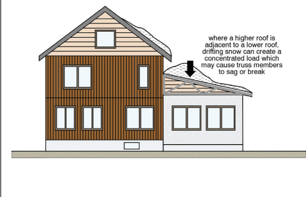
Drifting snow can cause truss sag/damage
