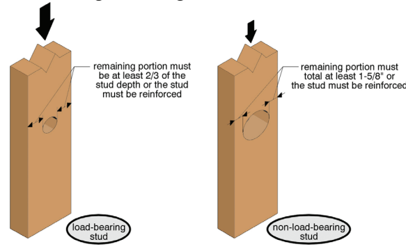
Stud notching and drilling
