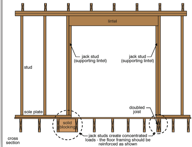
Support for jack studs on wide openings
