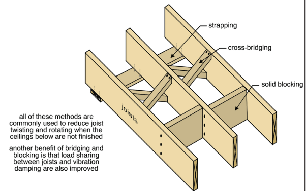
Strapping, bridging and blocking
